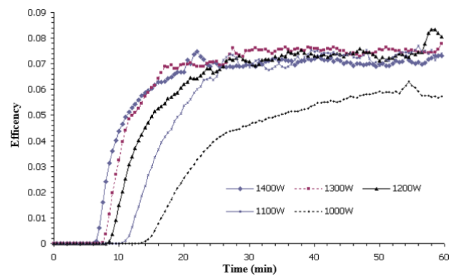
Fig. 10. TEG-RFA efficiency versus time for different power supply at 3 cm air gap.
