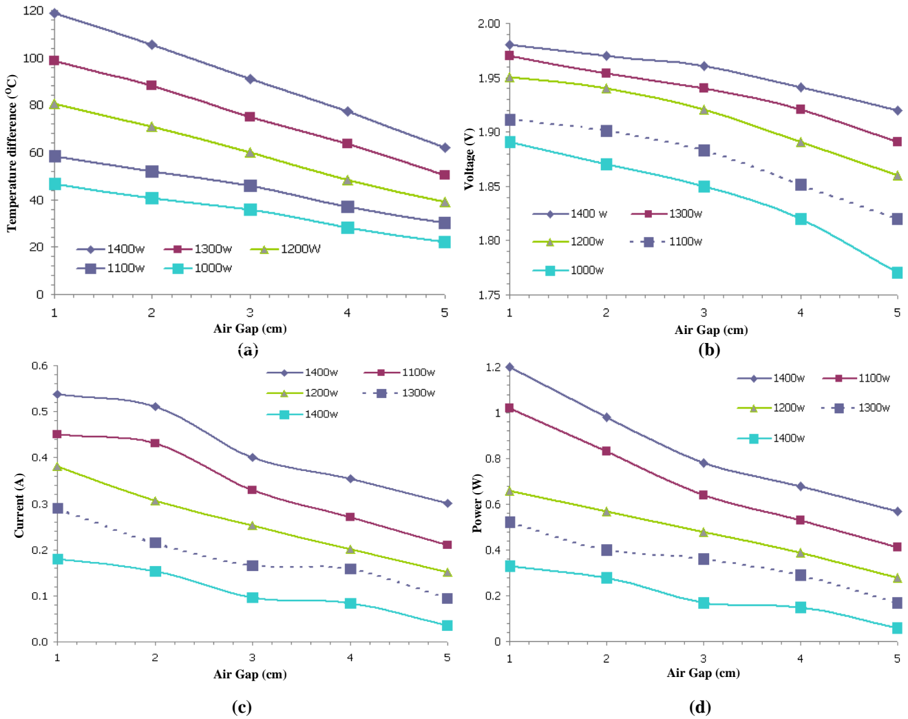
Fig. 8. Measured variations of (a) temperature difference between hot and cold sides of thermoelectric modules (b) generated electrical voltage (c) current (d) power for the different air gap spaces and different power supplied to the heated plate at steady conditions
