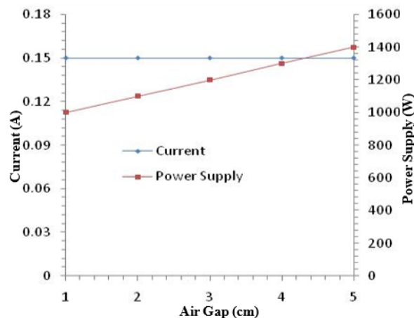
Fig. 9. Relationship between air gap space and power supplied to the heated plate to generate constant electrical current.
