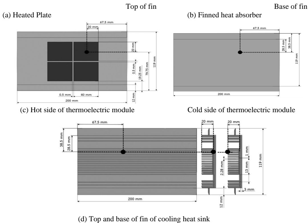
Fig.4. Positions of the temperature measurements: (a) Heated Plate (b) Finned heat absorber (c) Hot and cold sides of thermoelectric module (d) Top and base of fin of cooling heat sink.
