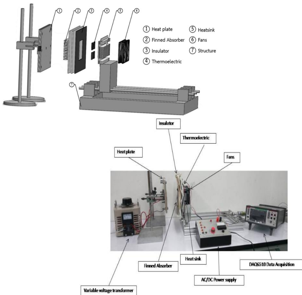
Fig. 3. Schematic of TEG-RFA (top) and experimental diagram and picture of the lab-scale setup (bottom).
