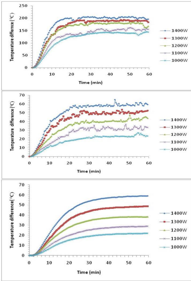
Fig.5. Variations of measured temperature difference between (top) heated plate and top of fin of heat absorber, (middle) top and base of fin of heat absorber and (bottom) hot and cold sides of thermoelectric module versus time for various electrical power supplied at 3 cm air gap.
