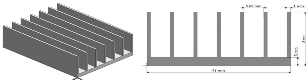
(a) Geometry and dimensions of finned heat absorber
