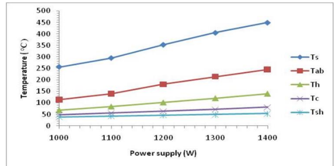
Fig. 6. Variations of measured temperatures of heated plate ( T_s ), base of fin of absorber ( T_{ab} ), hot ( T_h ) and cold ( T_c ) sides of thermoelectric module, and top of cooling heat sink ( T_{sh} ) for different electrical power supplied to the heater at 3 cm air gap space at steady conditions.
